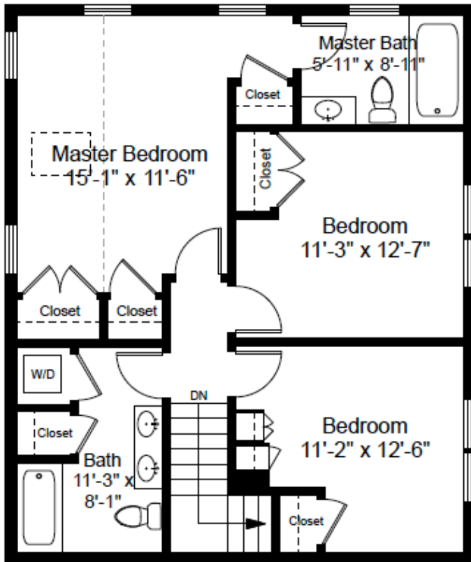
Second Floor Plan Ceiling Height = 11'-8"
