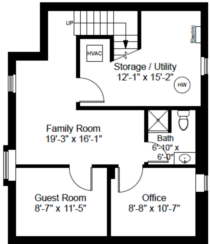
Lower Level Plan Ceiling Height = 7'-5"
